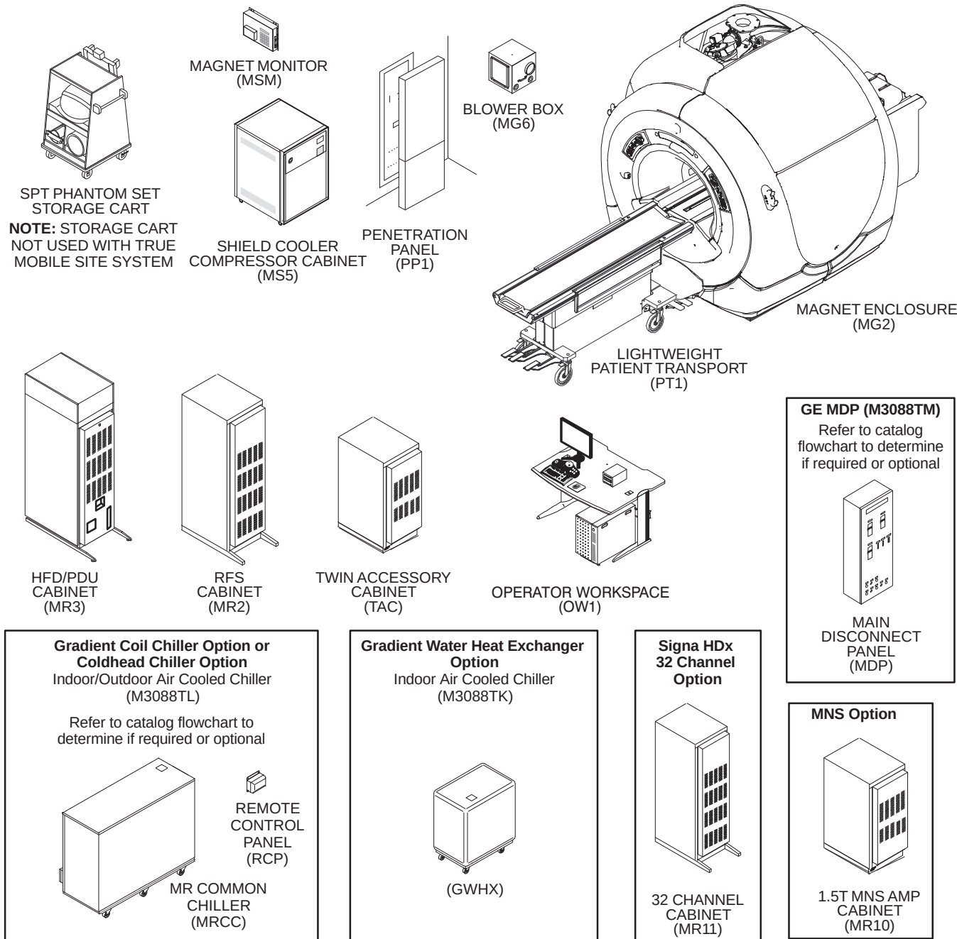
SIGNA HDx 1.5T TwinSpeed SYSTEM ILLUSTRATION 10-1
