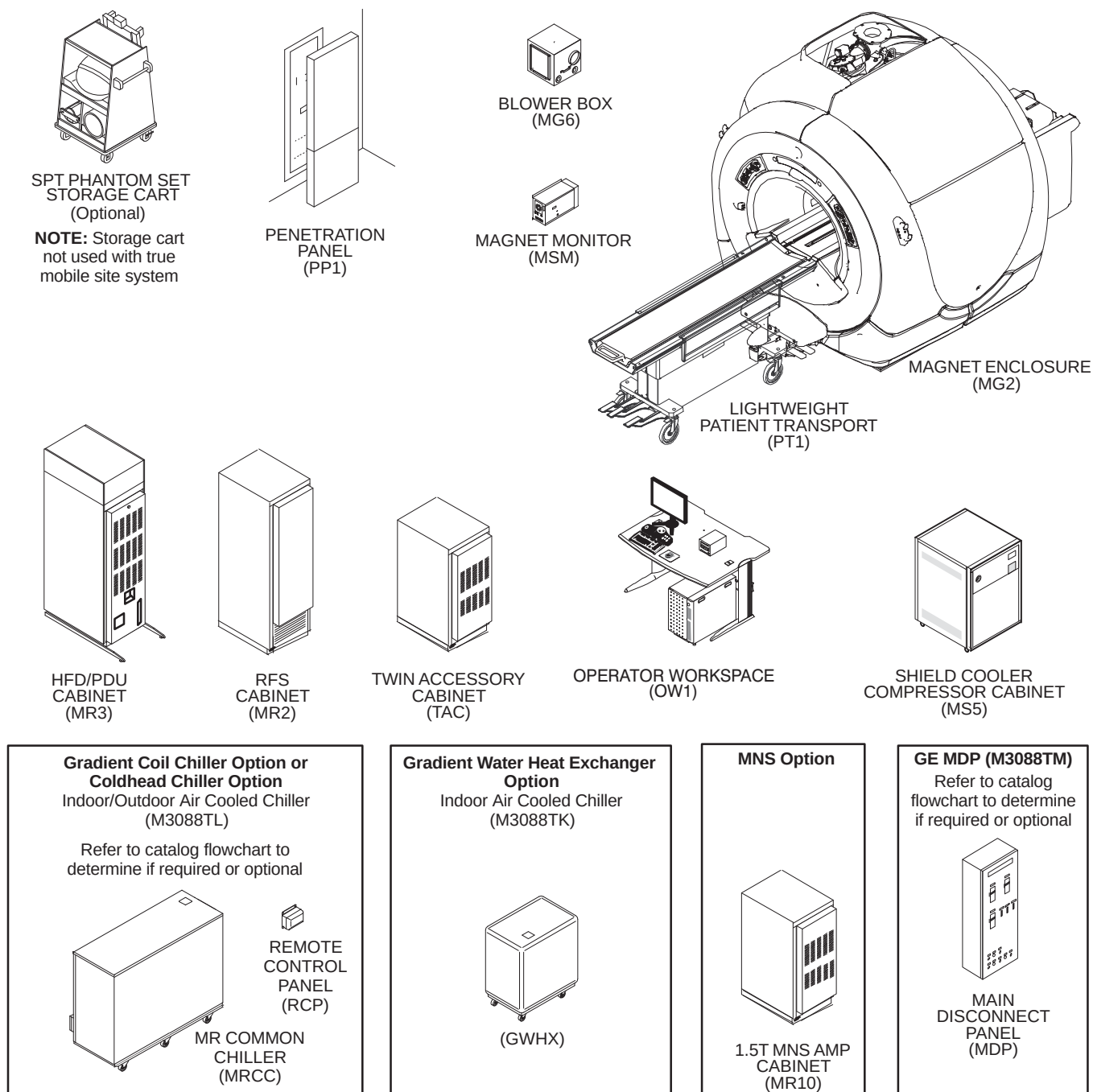
SIGNA EXCITE 1.5T SYSTEM ILLUSTRATION 1-1
