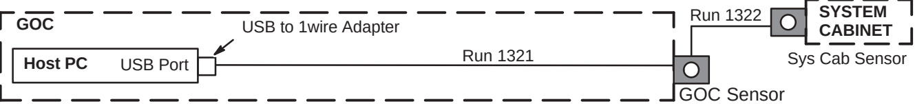
Environmental Sensors Block Diagram (Shipped after July 1, 2008)
